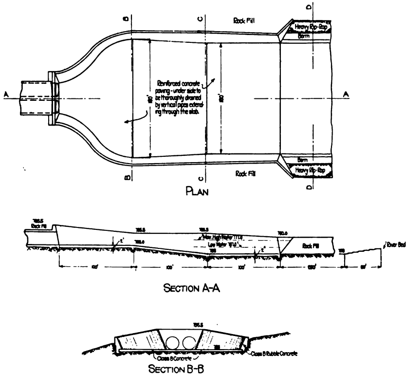
FIG. 44.—Stilling basin below the outlet of the proposed Dublin dam, for reducing the high conduit velocities to velocities that will not erode the natural river channel.
